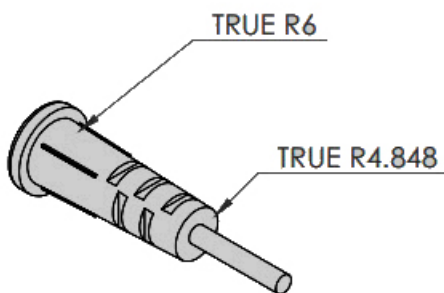
Socket taper profile
